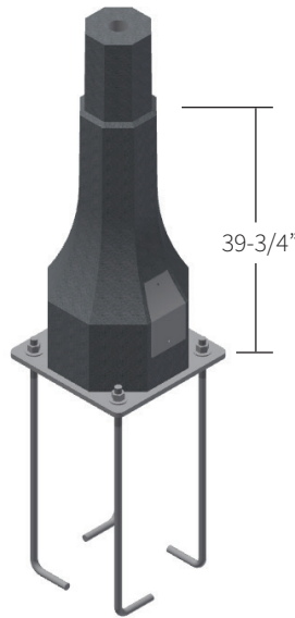
Elevation See Recommended "Capping Detail"
