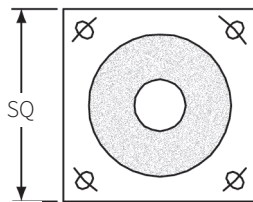
Std base plate prestressed to pole
