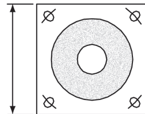
Std base plate prestressed to pole
